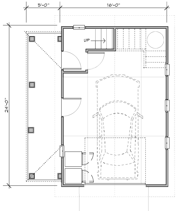
GARAGE PLAN
