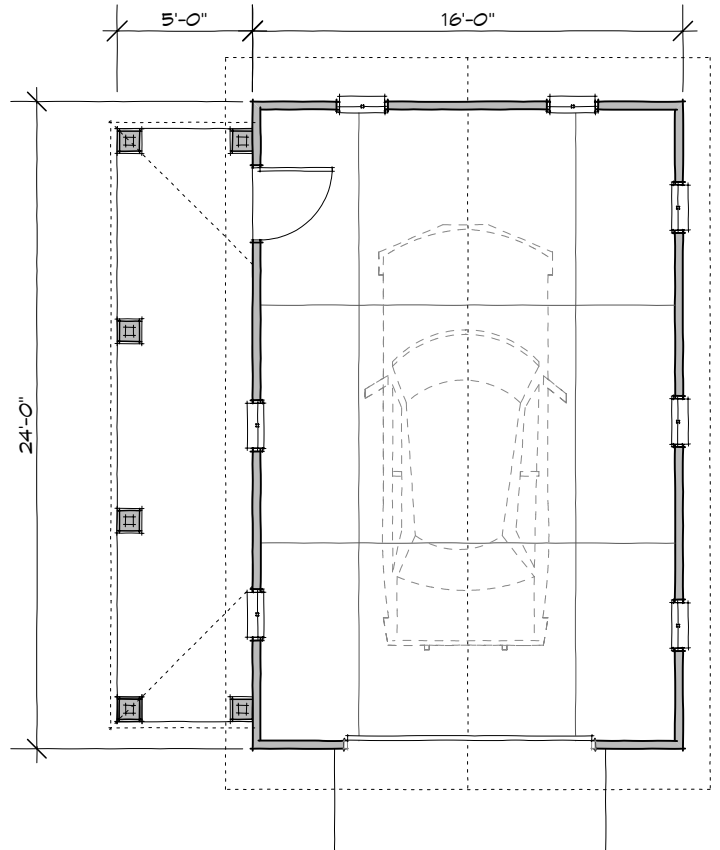
FLOOR PLAN
